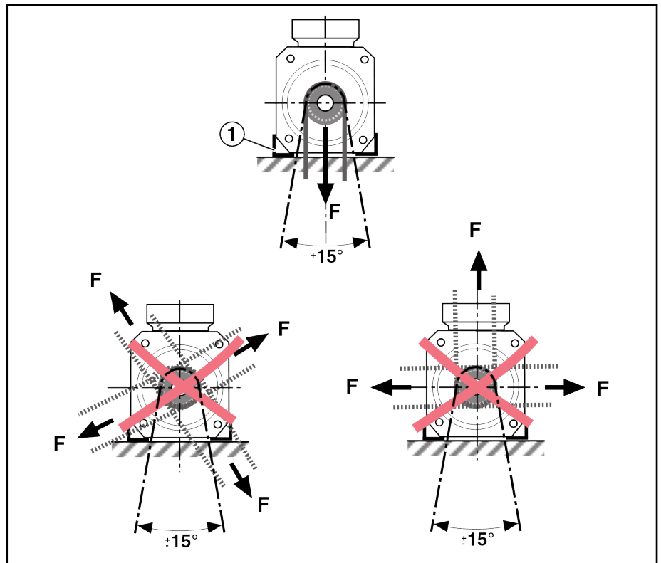
① Mounting feet
