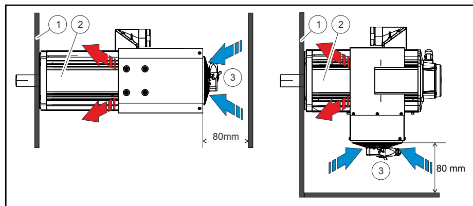
Fig. 9-16: Fan units, installation space, minimum distance
