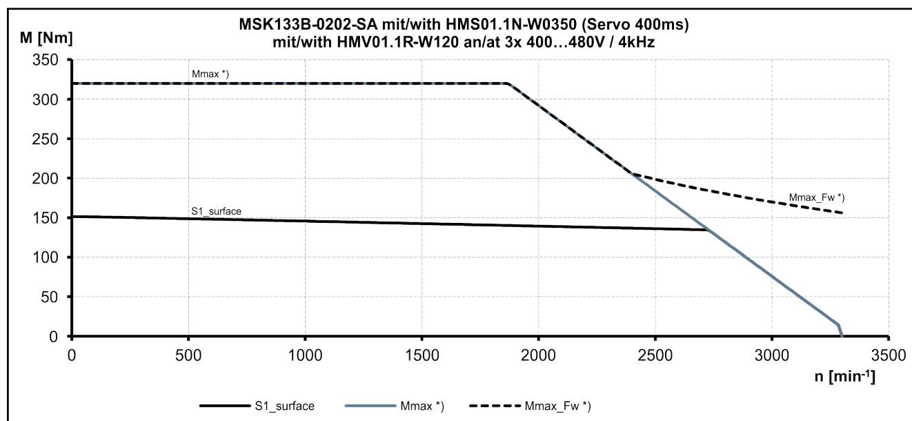
Fig. 4-80: Speed-torque characteristic curves
