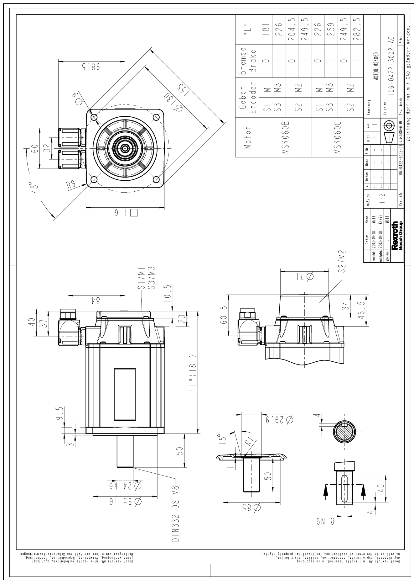
Fig. 5-5: MSK060 specification
