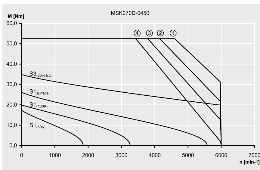
Fig. 4-29: Characteristic curves of an MSK070D-0450 motor
