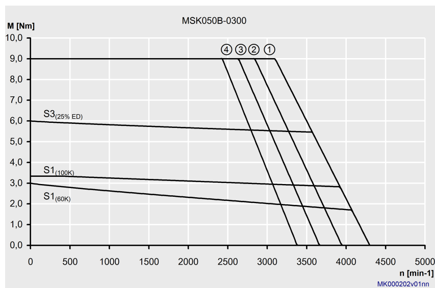
Fig. 4-10: Characteristic curves of an MSK050B-0300 motor
