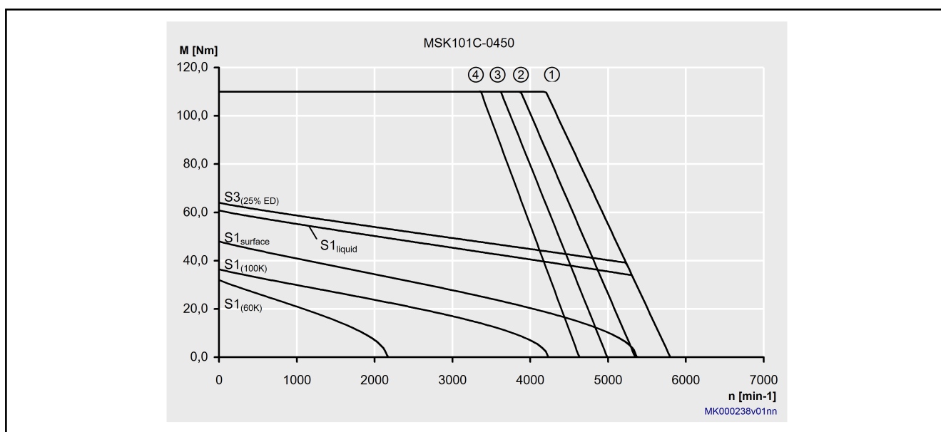
Fig. 4-68: Characteristic curve of a MSK101C-0450 motor
