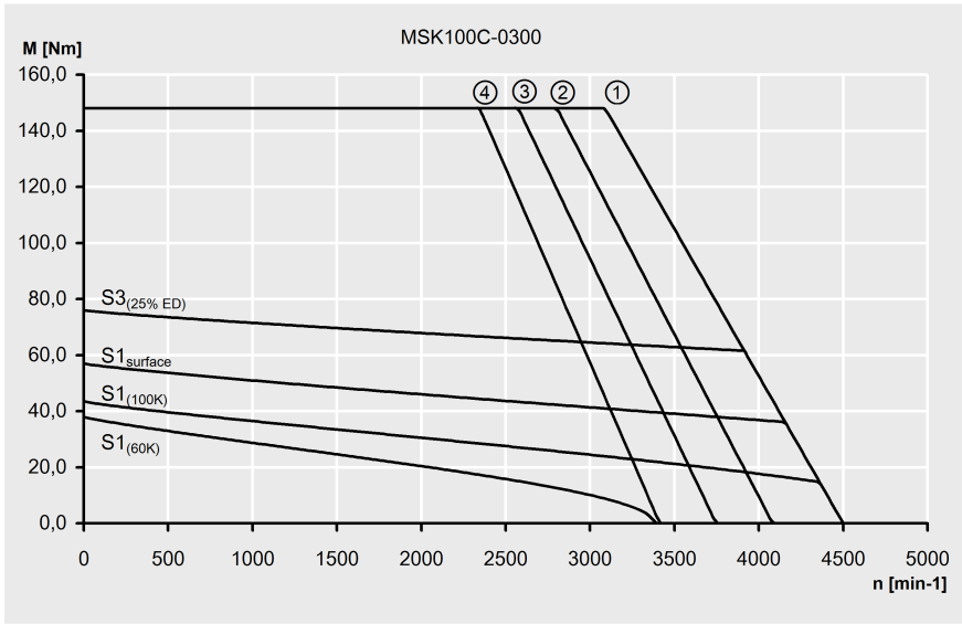
Fig. 4-61: Characteristic curve of a MSK100C-0300 motor
