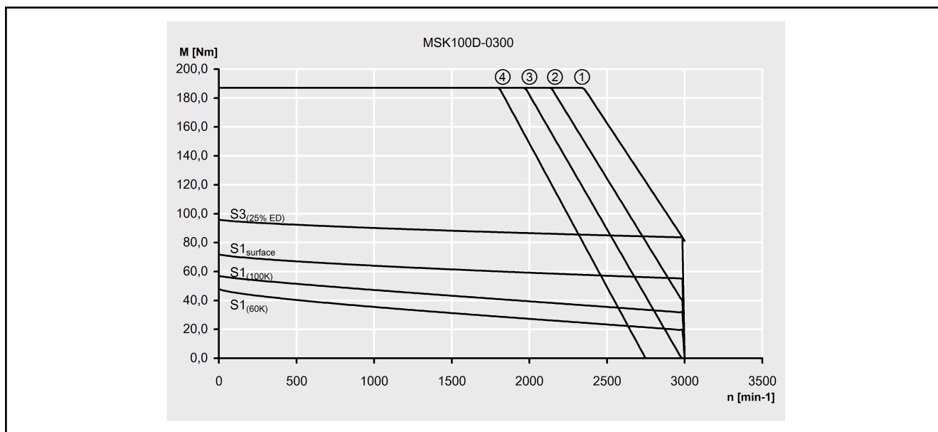
Fig. 4-64: Characteristic curve of a MSK100D-0300 motor
