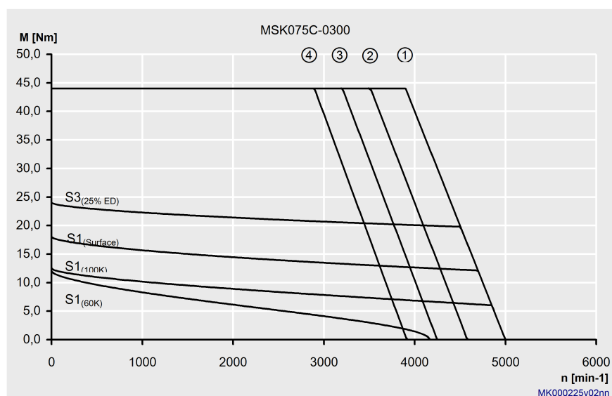
Fig. 4-43: Motor characteristic curve MSK075C-300
