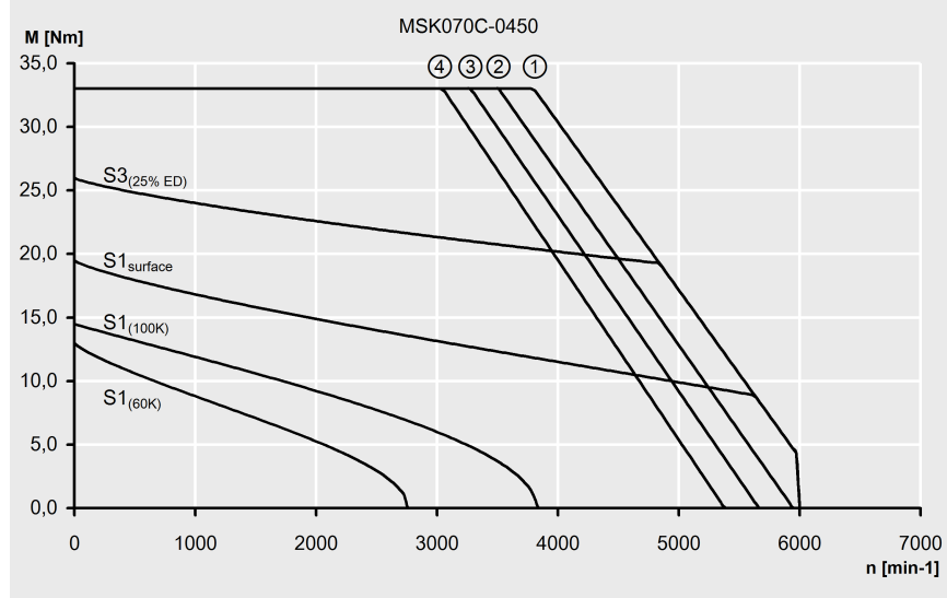
Fig. 4-26: Characteristic curves of an MSK070C-0450 motor
