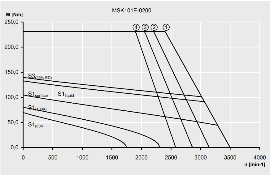
Fig. 4-72: Characteristic curve of a MSK101E-0200 motor
