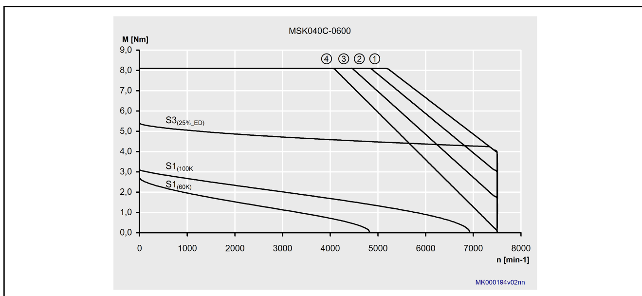
Fig. 4-8: Characteristic curves of an MSK040C-0600 motor
