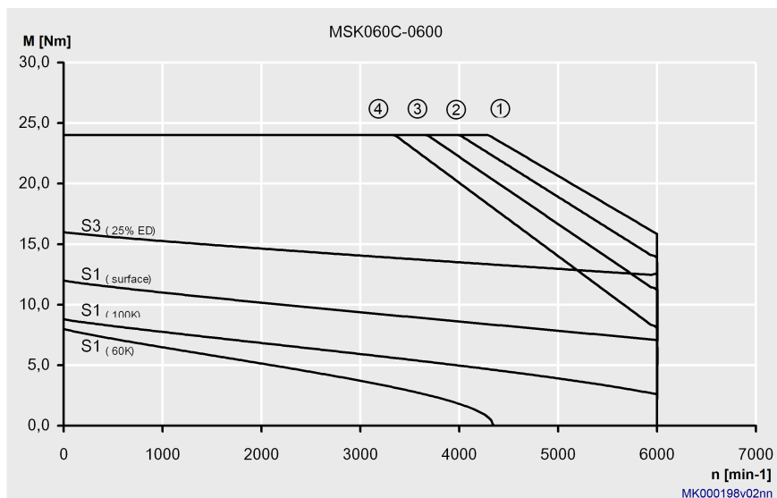
Fig. 4-19: Characteristic curves of an MSK060C-0600 motor
