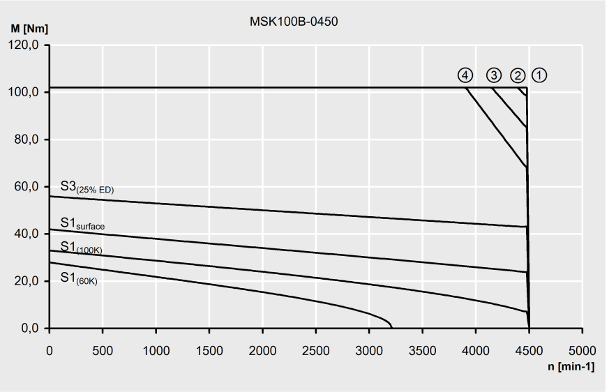
Fig. 4-59: Characteristic curve of a MSK100B-0450 motor
