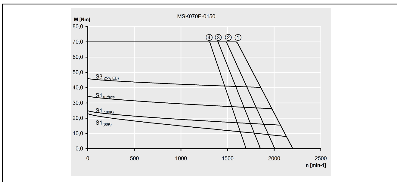
Fig. 4-30: Characteristic curves of an MSK070E-0150 motor
