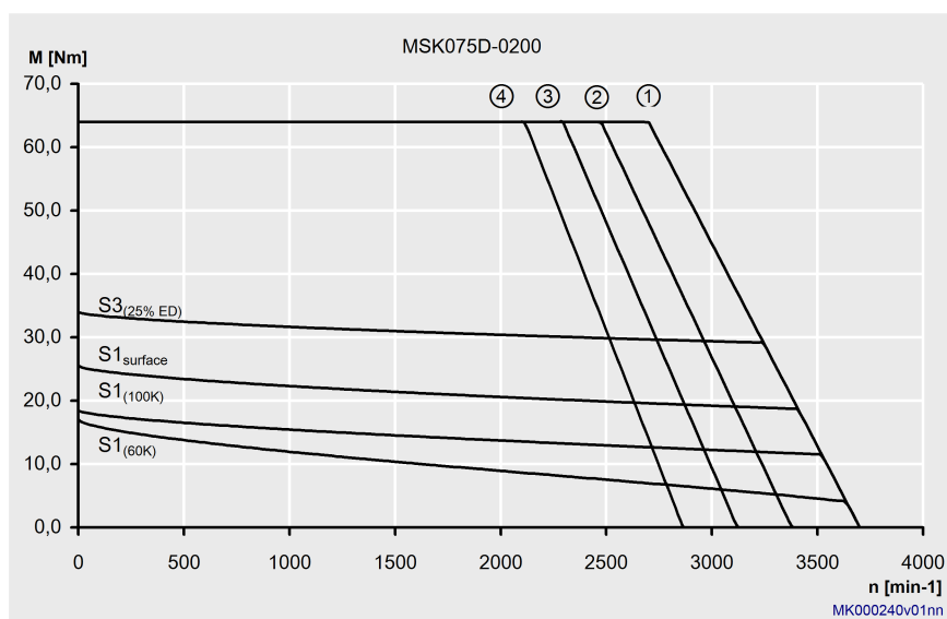
Fig. 4-45: Motor characteristic curve MSK075D-0200
