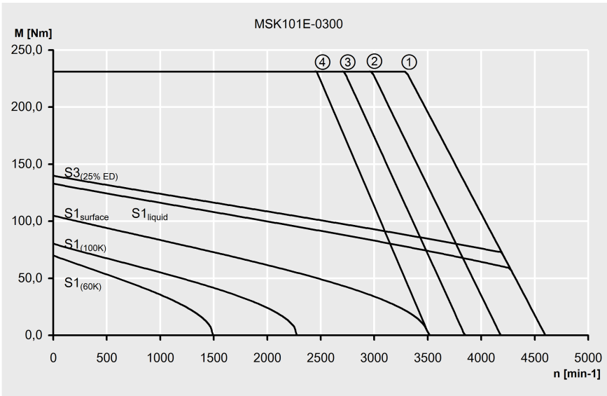
Fig. 4-73: Characteristic curve of a MSK101E-300 motor
