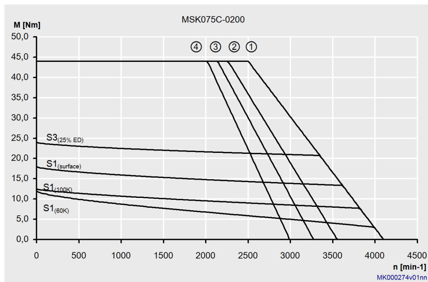
Fig. 4-42: Motor characteristic curve MSK075C-0200
