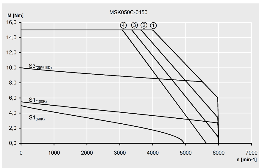
Fig. 4-14: Characteristic curves of an MSK050C-0450 motor
