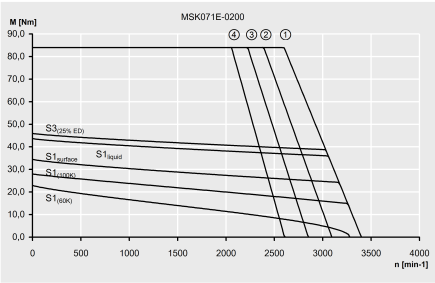
Fig. 4-39: Characteristic curves of an MSK071E-0200 motor
