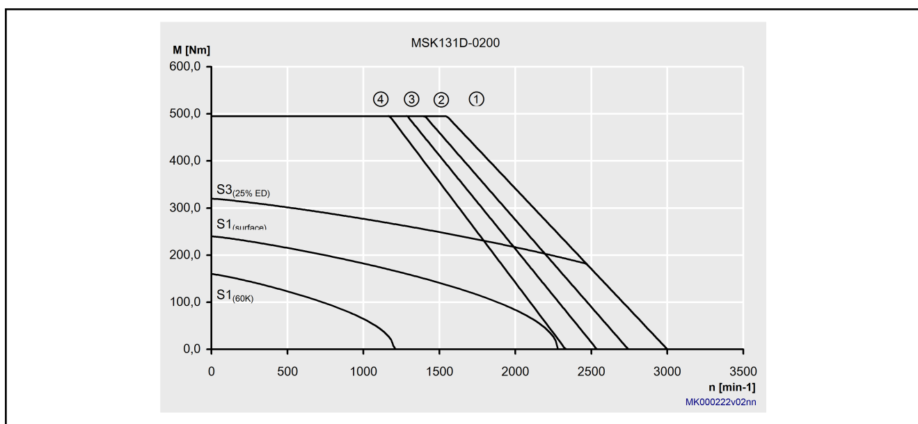
Fig. 4-79: Characteristic curve of a MSK131D-0200 motor
