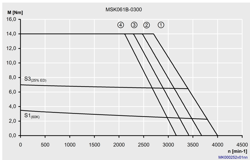
Fig. 4-20: Characteristic curves of an MSK061B-0300 motor
