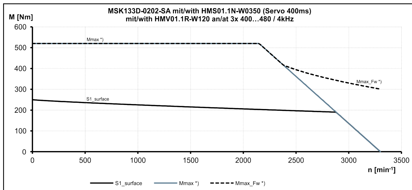
Fig. 4-88: Speed-torque characteristic curves
