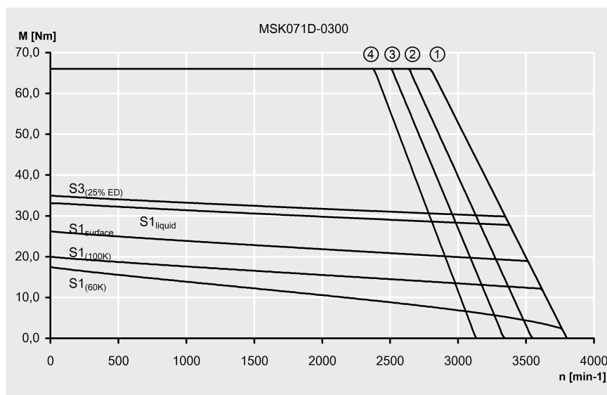
Fig. 4-37: Characteristic curves of an MSK071D-0300 motor
