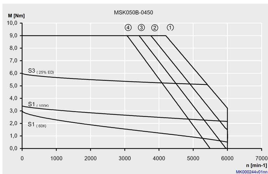
Fig. 4-11: Characteristic curves of an MSK050B-0450 motor
