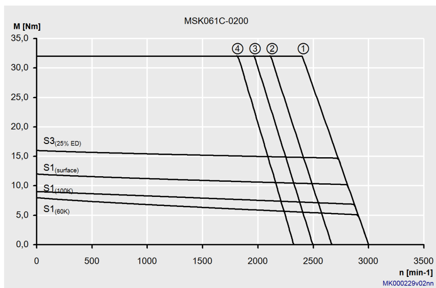
Fig. 4-21: Characteristic curves of an MSK061C-0200 motor
