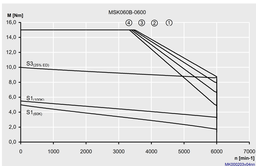
Fig. 4-17: Characteristic curves of an MSK060B-0600 motor
