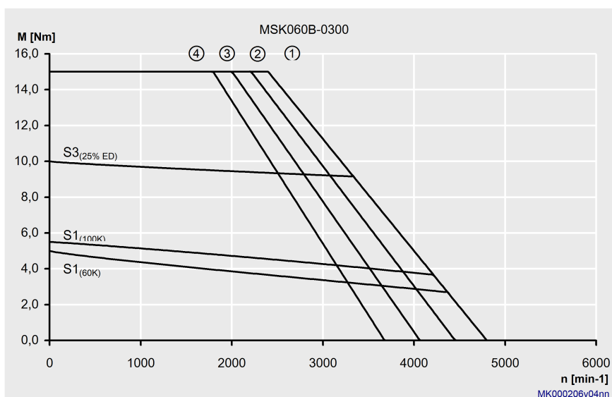
Fig. 4-16: Characteristic curves of an MSK060B-0300 motor
