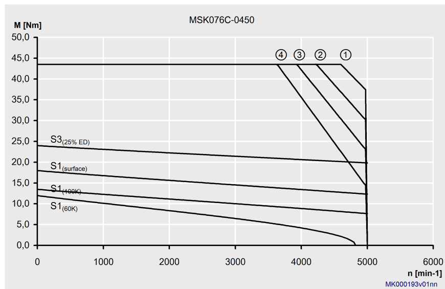
Fig. 4-52: Characteristic curves of an MSK076C-0450 motor
