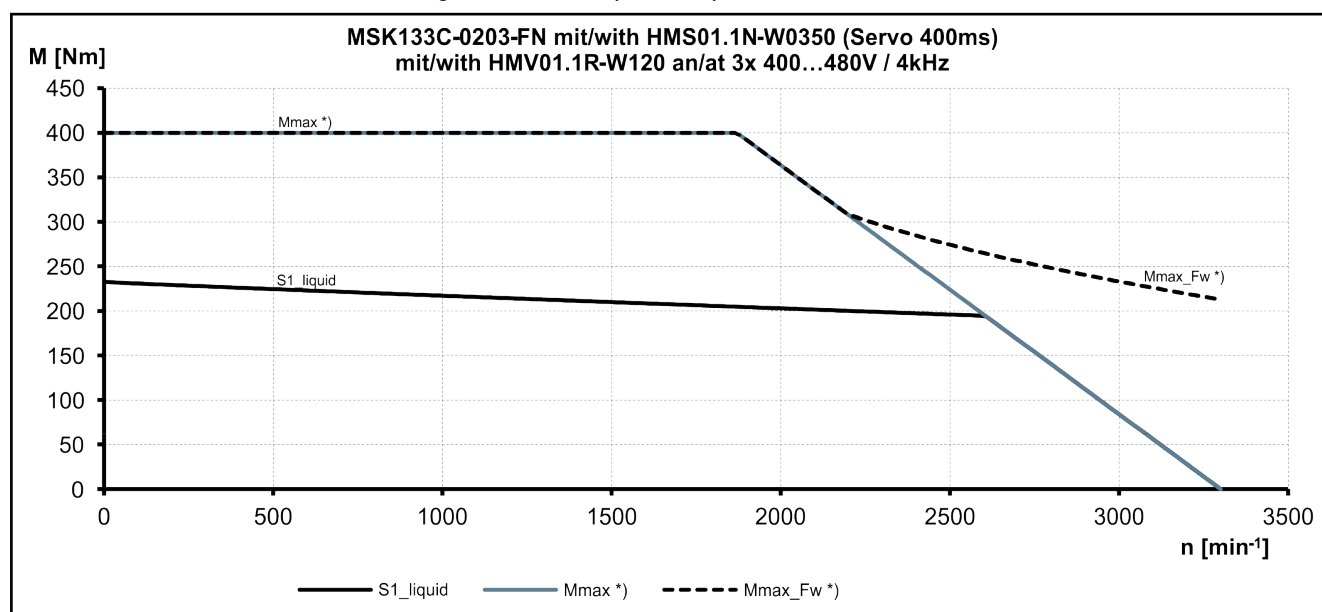
Fig. 4-86: Speed-torque characteristic curves
