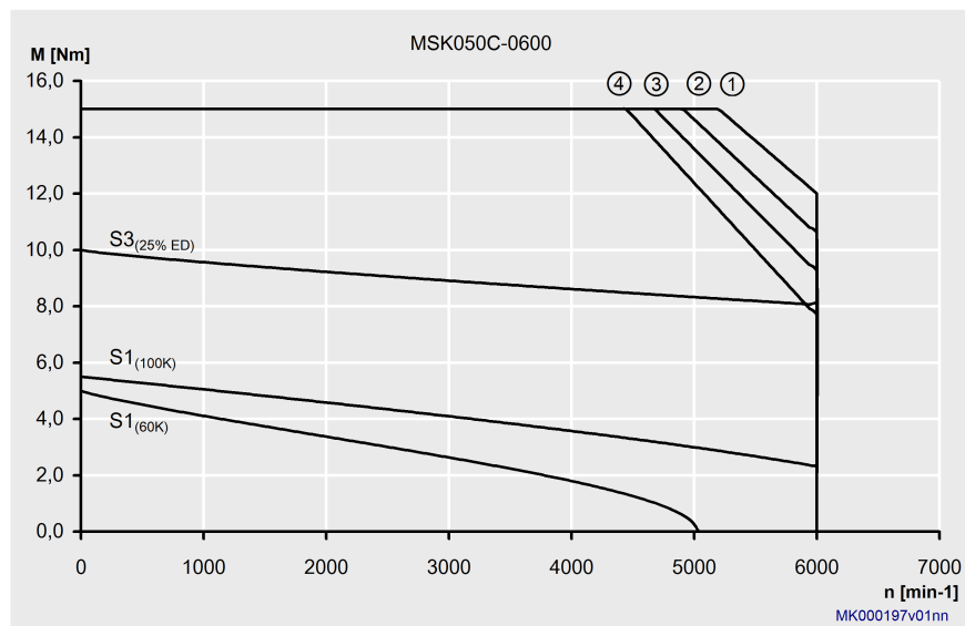
Fig. 4-15: Characteristic curves of an MSK050C-0600 motor
