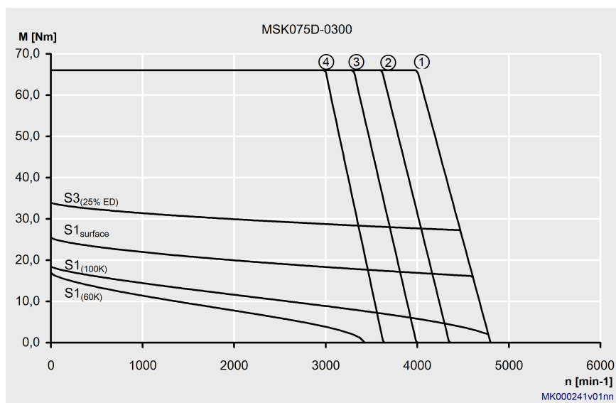
Fig. 4-46: Motor characteristic curve MSK075D-0300
