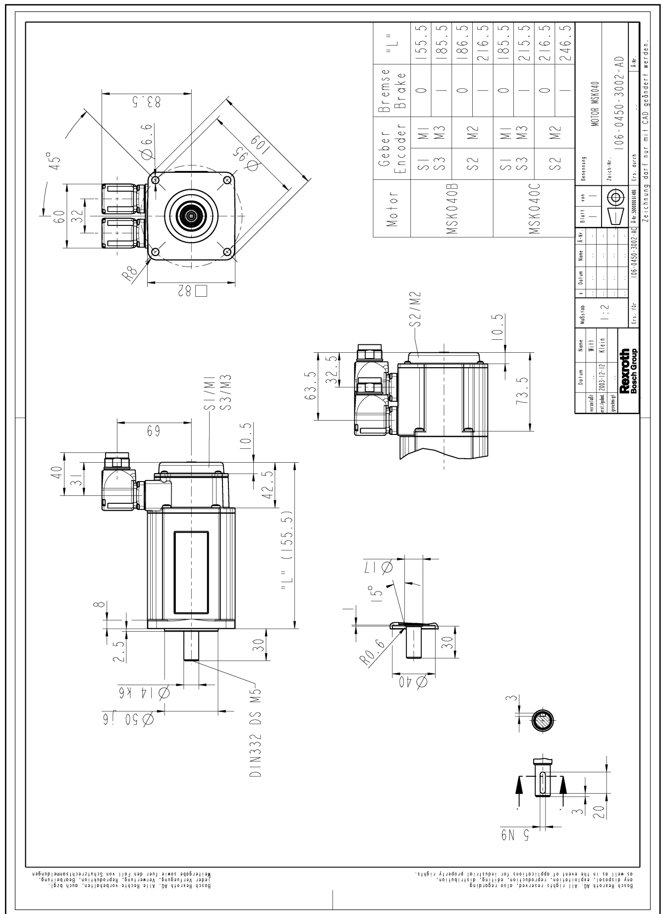
Fig. 5-2: MSK040 specification
