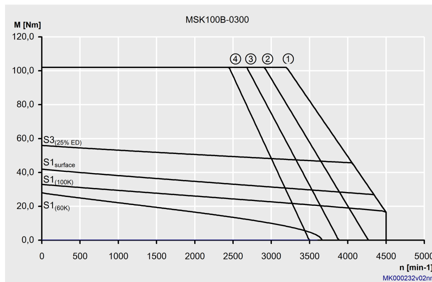
Fig. 4-57: Characteristic curve of a MSK100B-0300 motor
