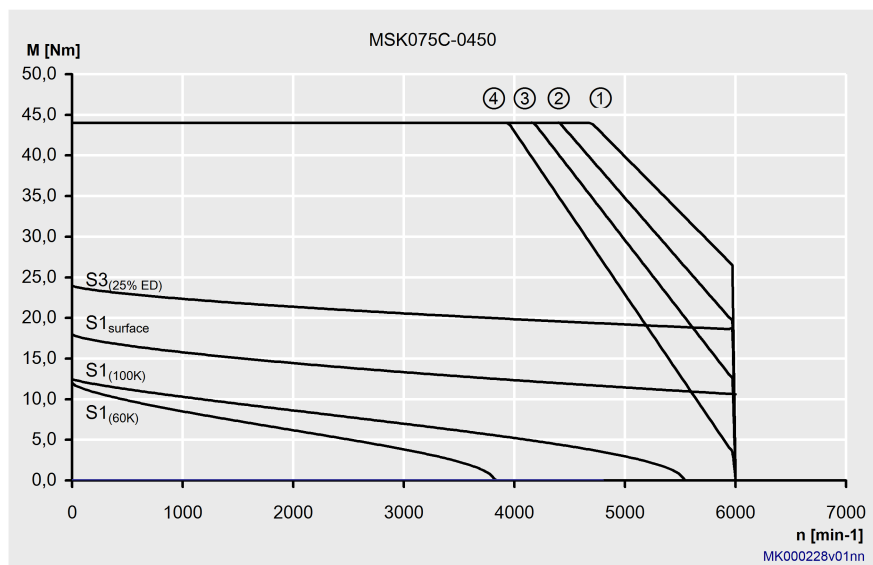
Fig. 4-44: Motor characteristic curve MSK075C-0450
