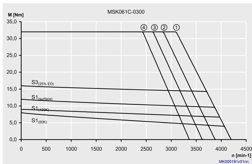
Fig. 4-22: Characteristic curves of an MSK061C-0300 motor
