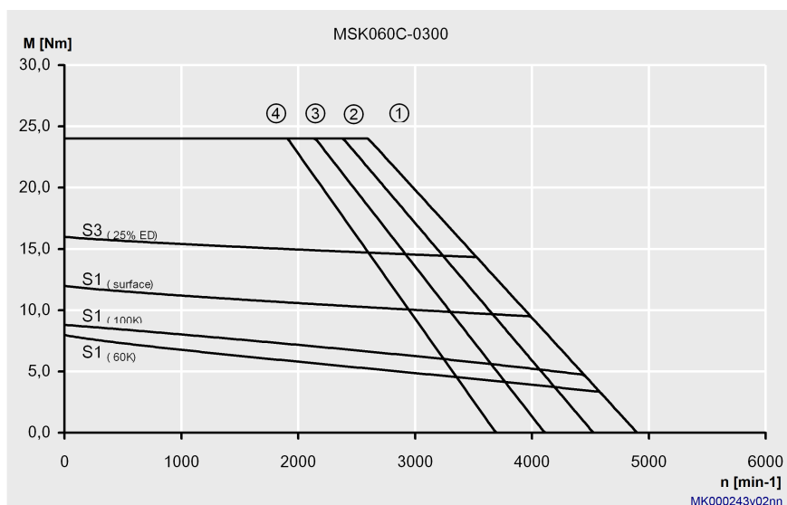
Fig. 4-18: Characteristic curves of an MSK060C-0300 motor
