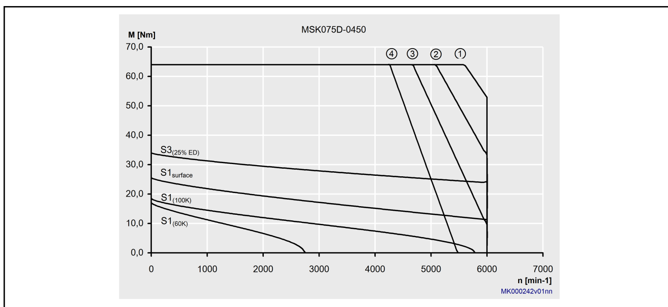
Fig. 4-47: Motor characteristic curve MSK075D-0450
