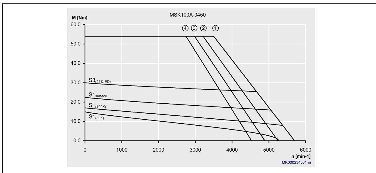
Fig. 4-55: Characteristic curve of a MSK100A-0450 motor
