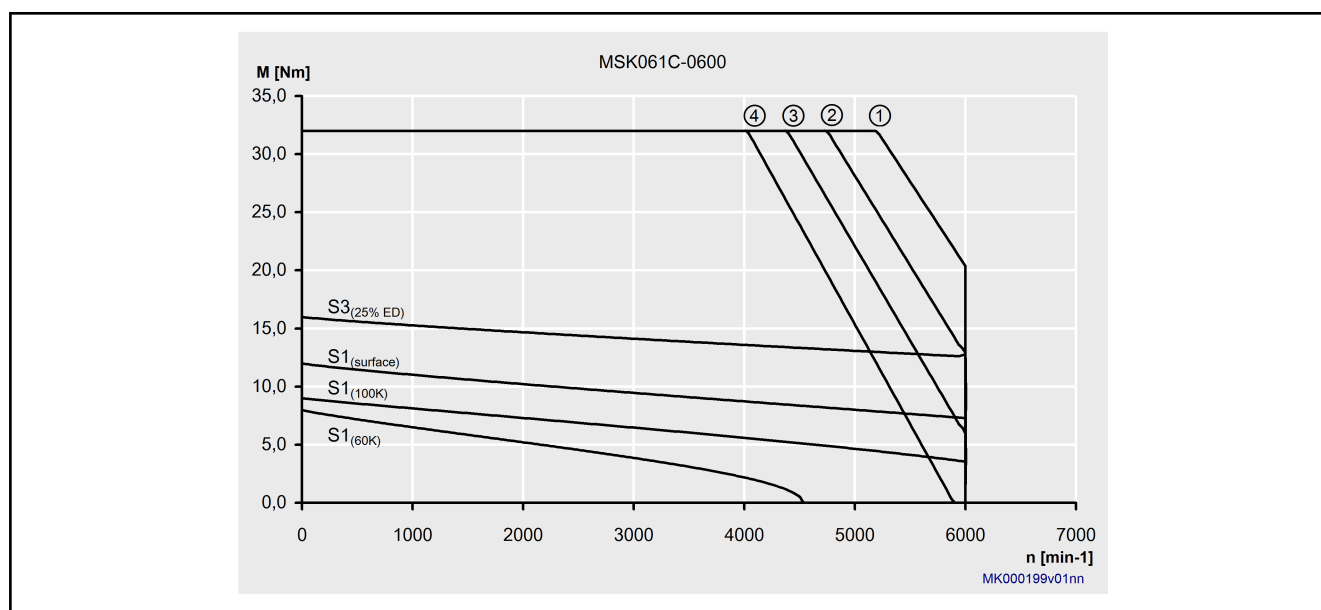
Fig. 4-23: Characteristic curves of an MSK061C-0600 motor
