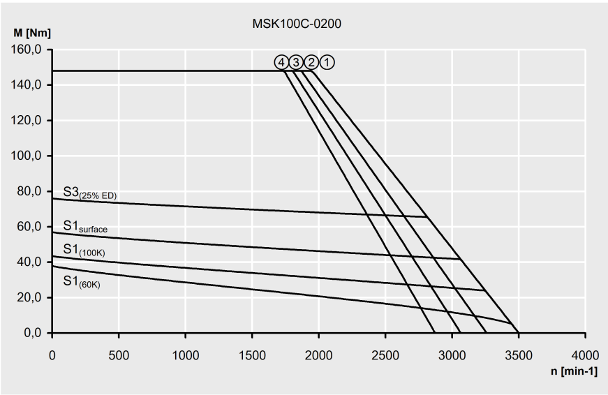
Fig. 4-60: Characteristic curve of a MSK100C-0200 motor
