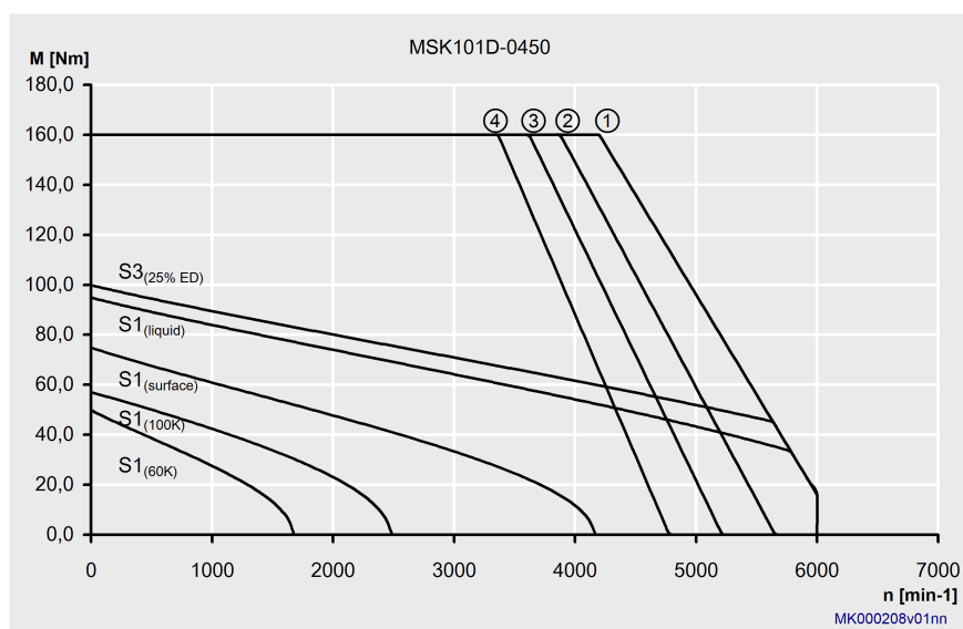
Fig. 4-71: Characteristic curve of a MSK101D-0450 motor
