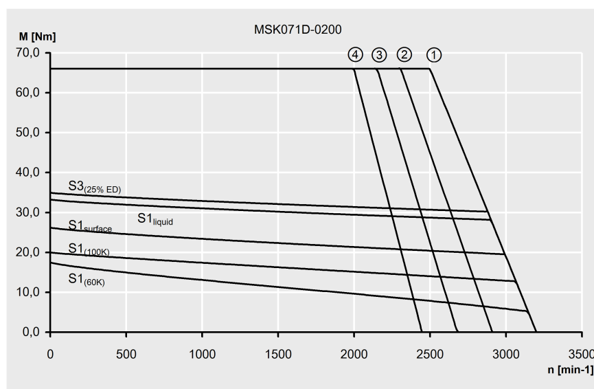
Fig. 4-36: Characteristic curves of an MSK071D-0200 motor
