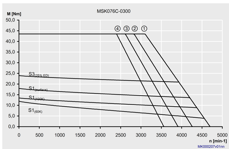
Fig. 4-51: Characteristic curves of an MSK076C-0300 motor
