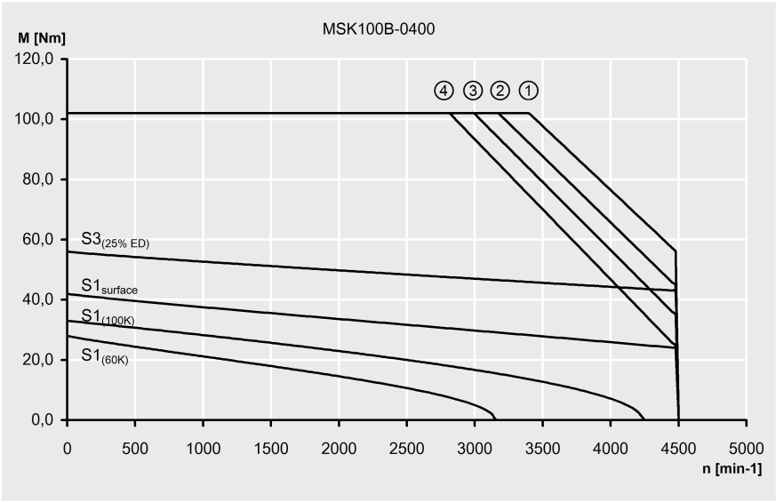
Fig. 4-58: Characteristic curve of a MSK100B-0400 motor
