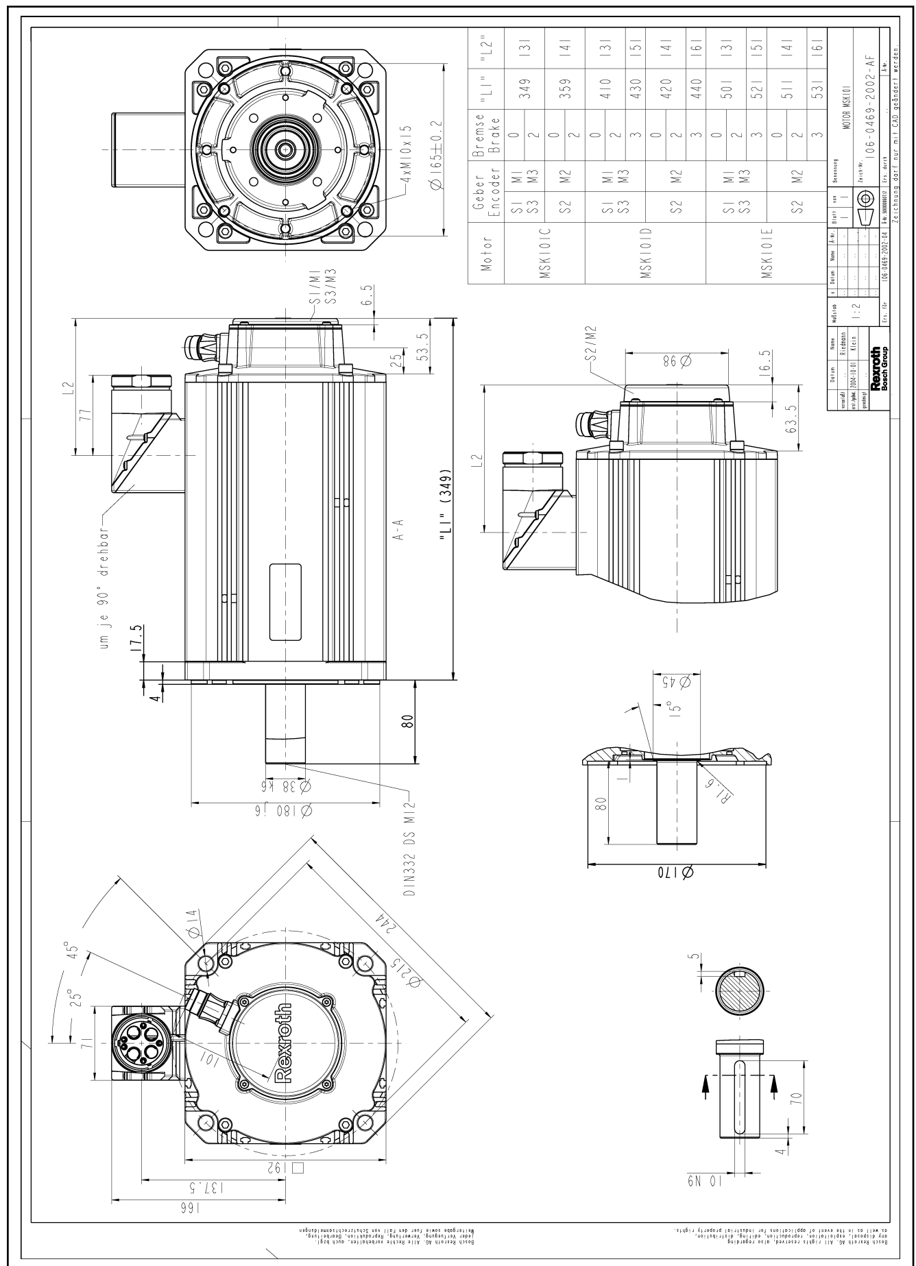
Fig. 5-28: MSK101 specification
