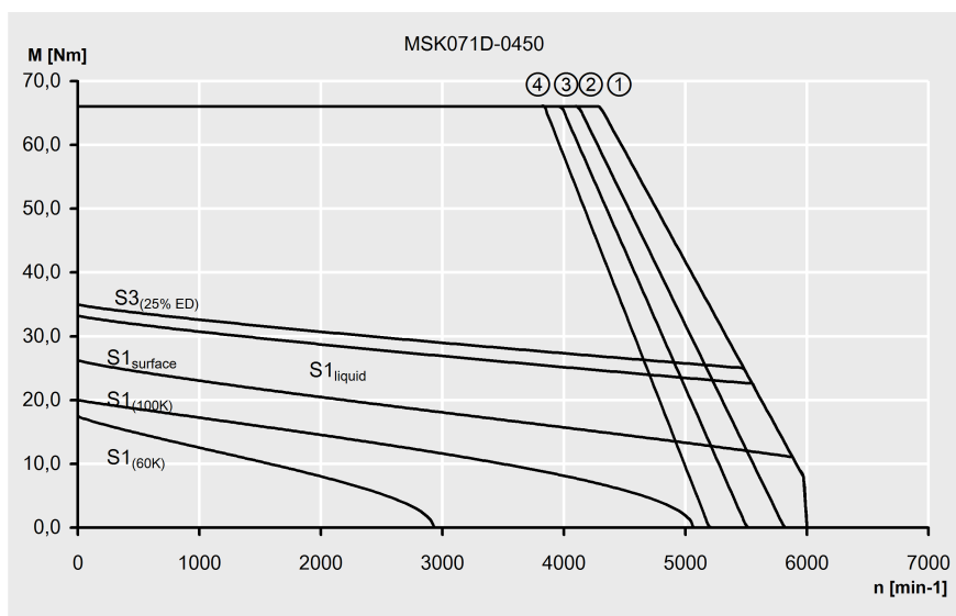
Fig. 4-38: Characteristic curves of an MSK071D-0450 motor
