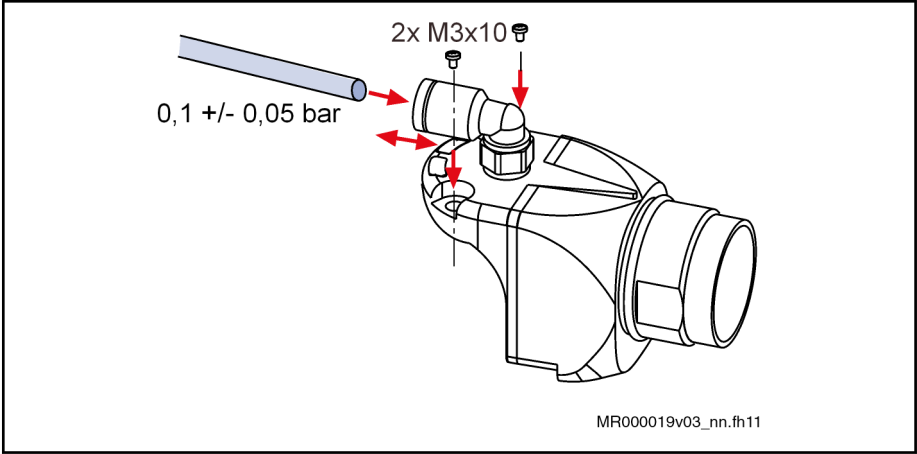
Fig. 7-9: RGS1000 with sealing air connection
