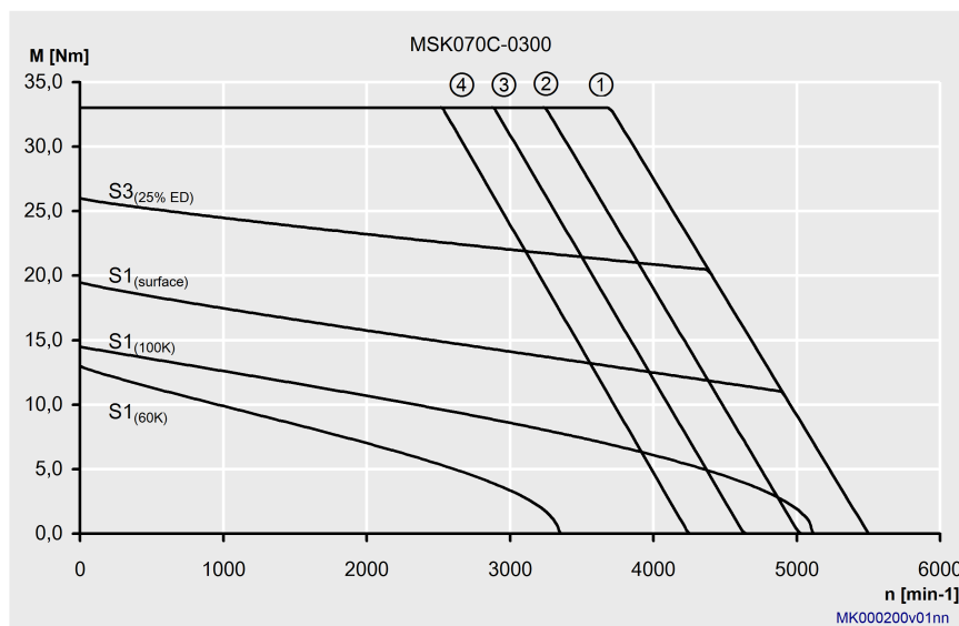
Fig. 4-25: Characteristic curves of an MSK070C-0300 motor
