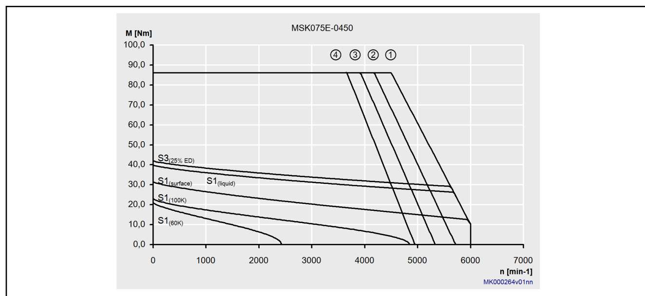
Fig. 4-50: Motor characteristic curve MSK075C-0450
