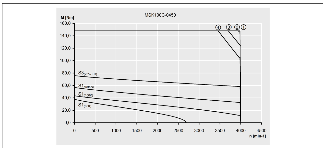
Fig. 4-62: Characteristic curve of a MSK100C-0450 motor
