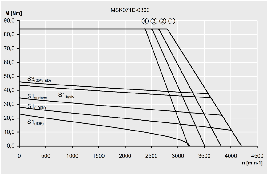
Fig. 4-40: Characteristic curves of an MSK071E-0300 motor
