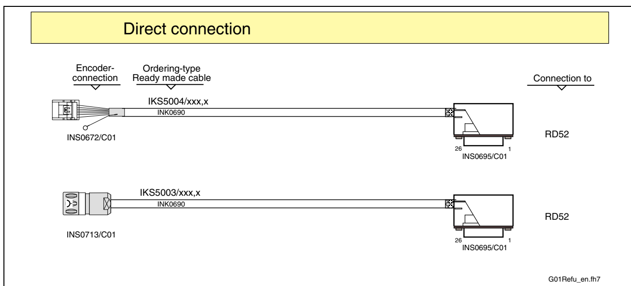
Fig. 17-16: Encoder cable MKD - REFUDRIVE RD52
