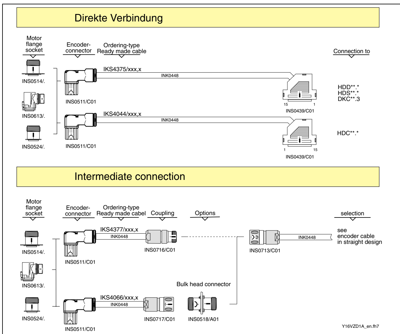
Fig. 17-15: Encoder cable (Connector angled) for MKD025, -112
