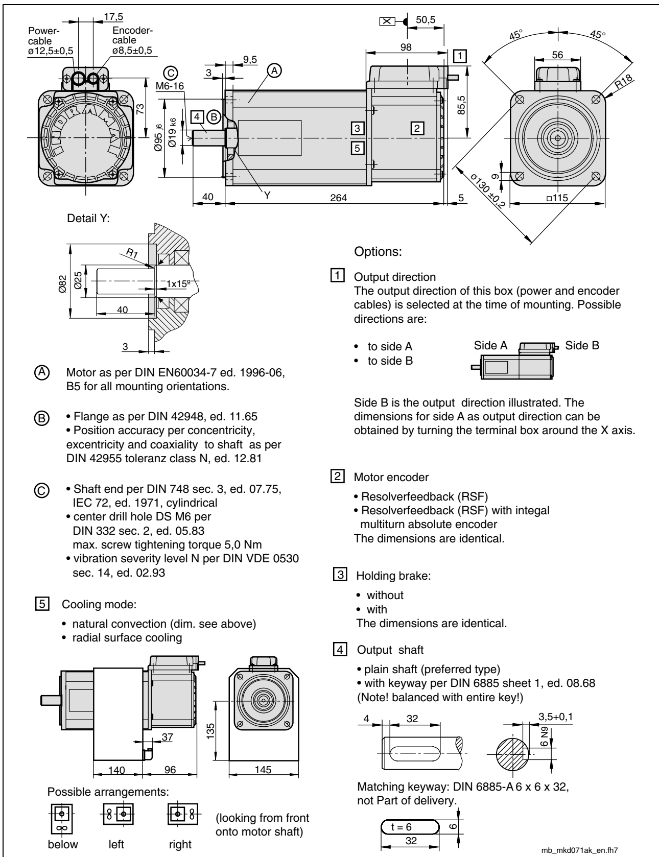
Fig. 8-9: Dimensional data MKD071 (holding brake 1)
