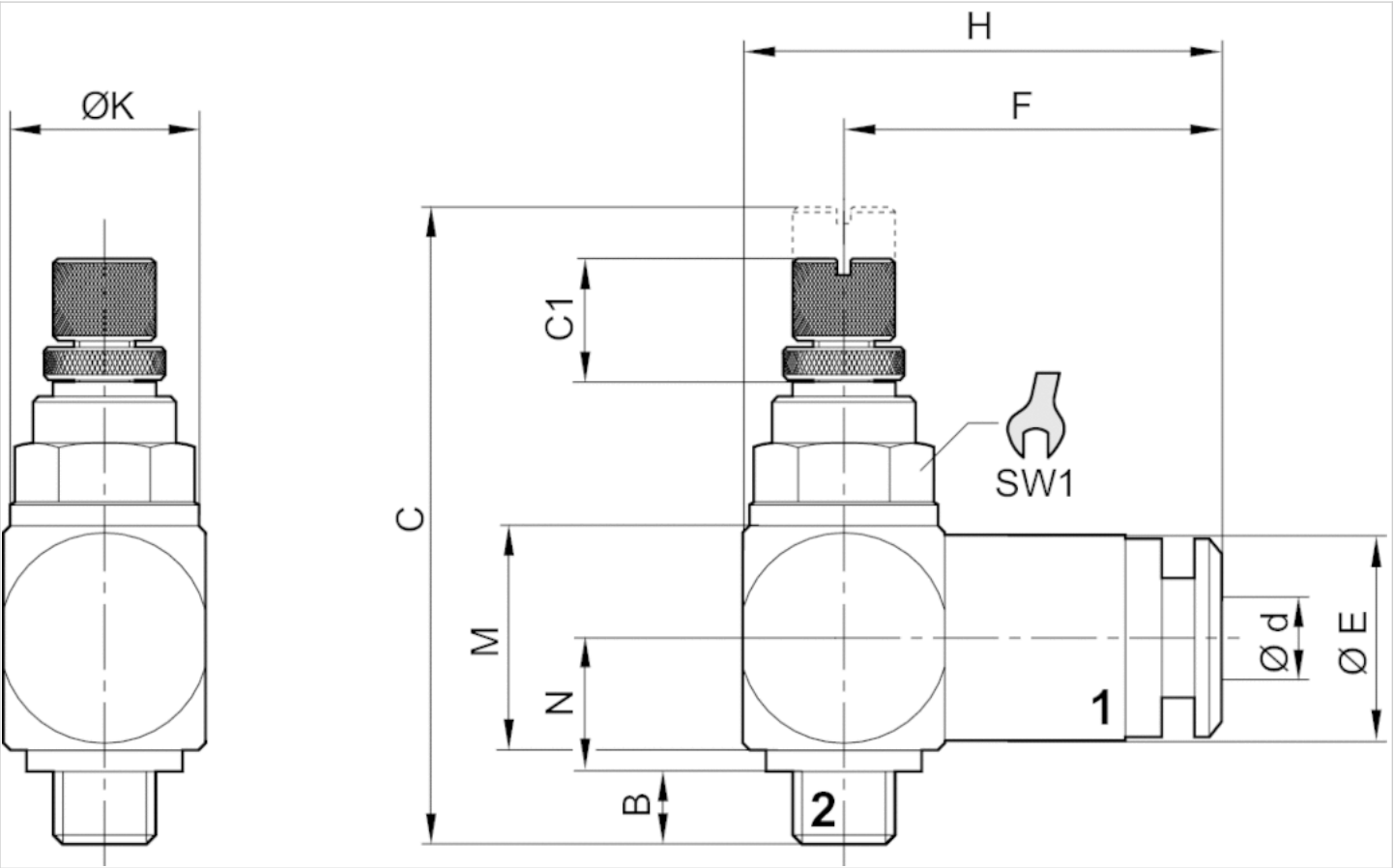
Throttle setting via knurled bolt
