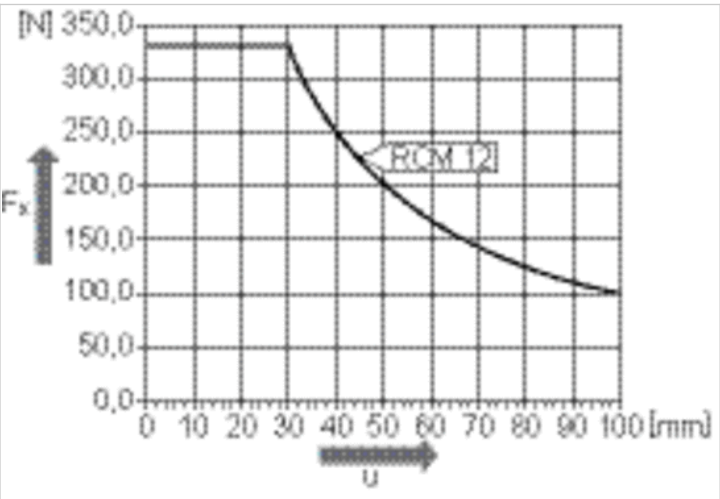
Maximum permissible axial force F_x [N] as a function of u [mm] RCM 12
