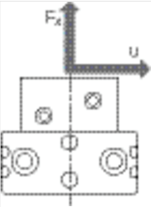
Maximum permissible axial force F_x [N] as a function of u [mm] RCM 12
