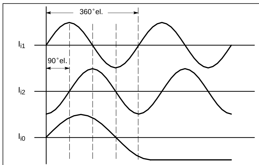
Signal diagram for measuring system with sinusoidal current signals
