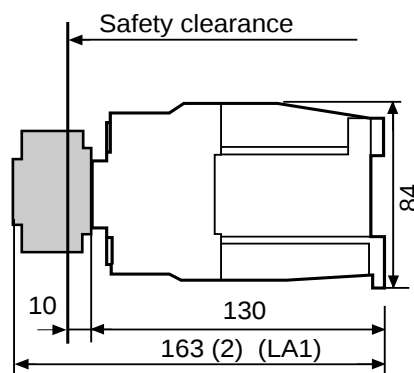
Figure 7.7: Dynamic brake contactor
