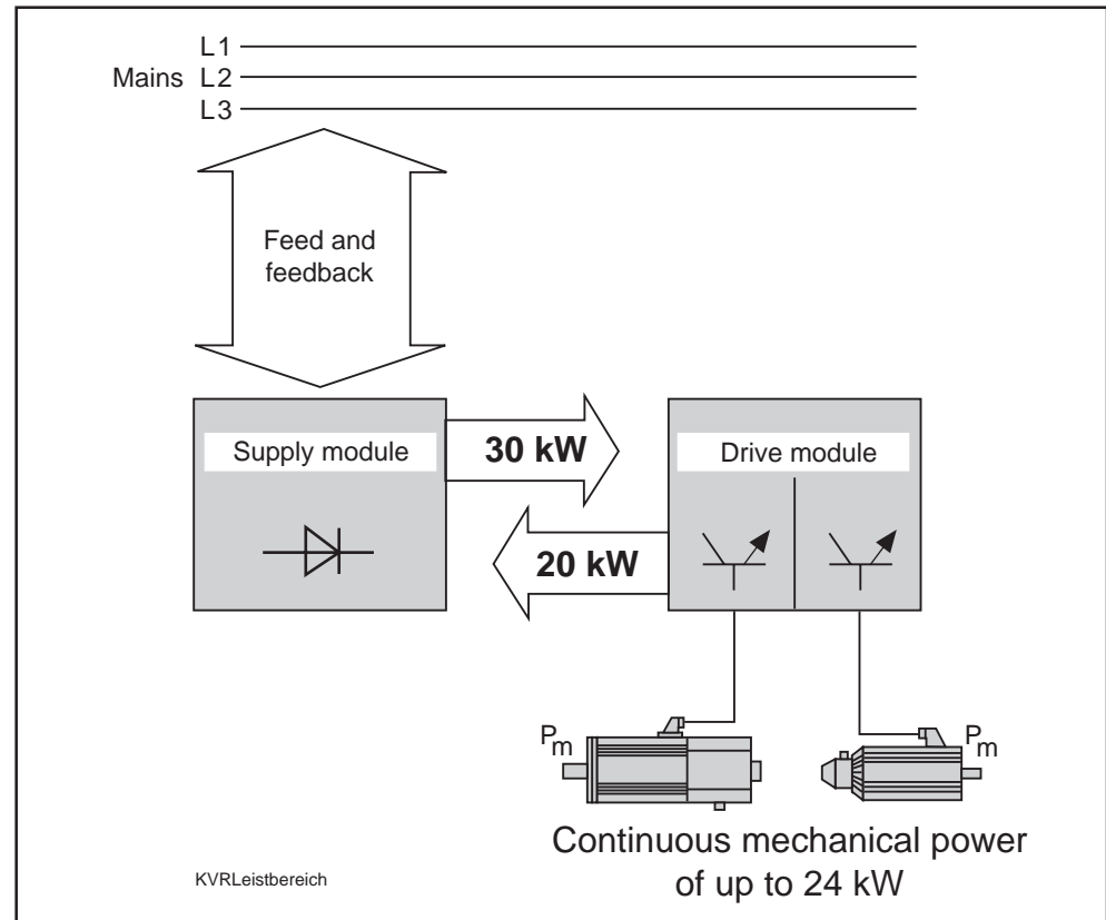
Figure 2.1: The power range for KDV 4 supply module applications.
