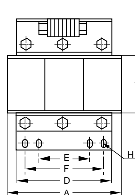
Side Mounted Version for Walls Type DST.../L
