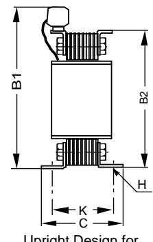
Upright Design for Floor Mounting Type DST.../S
