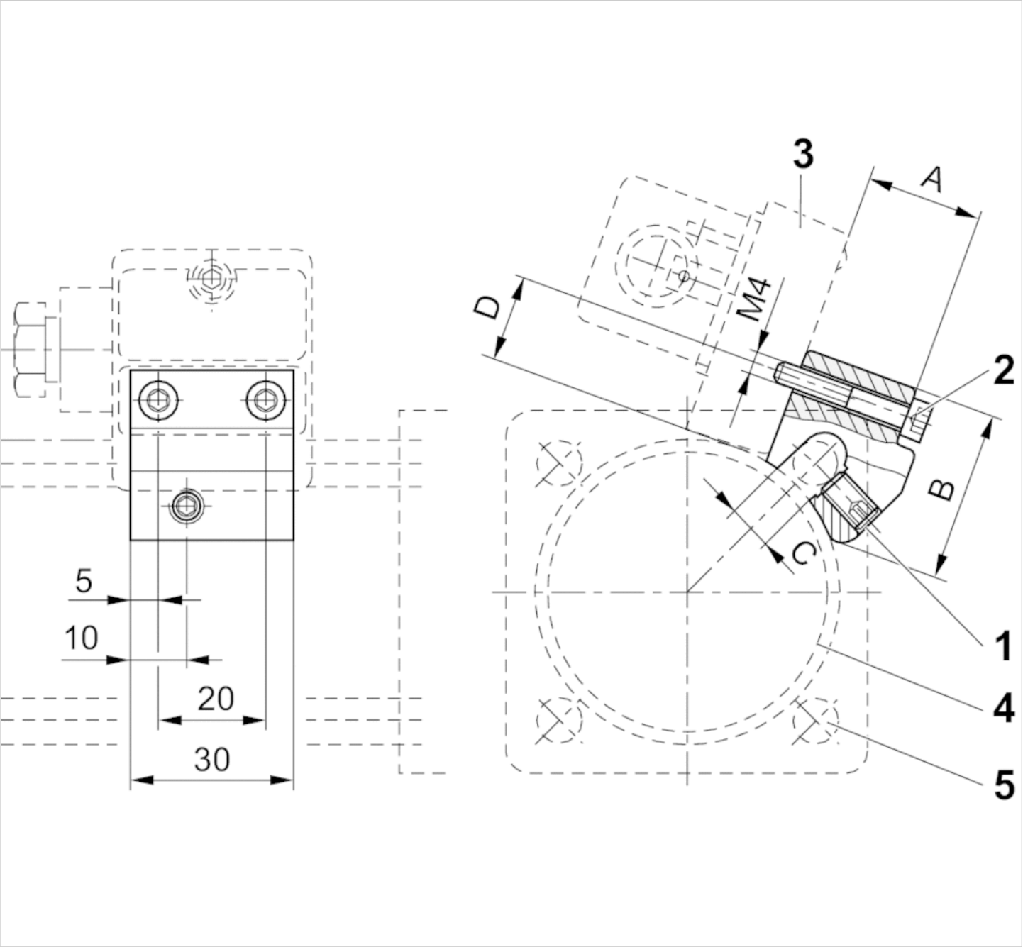
1) Clamping threaded pin 2) Mounting screw for sensor 3) Sensor 4) Cylinder profile 5) Tie rod
