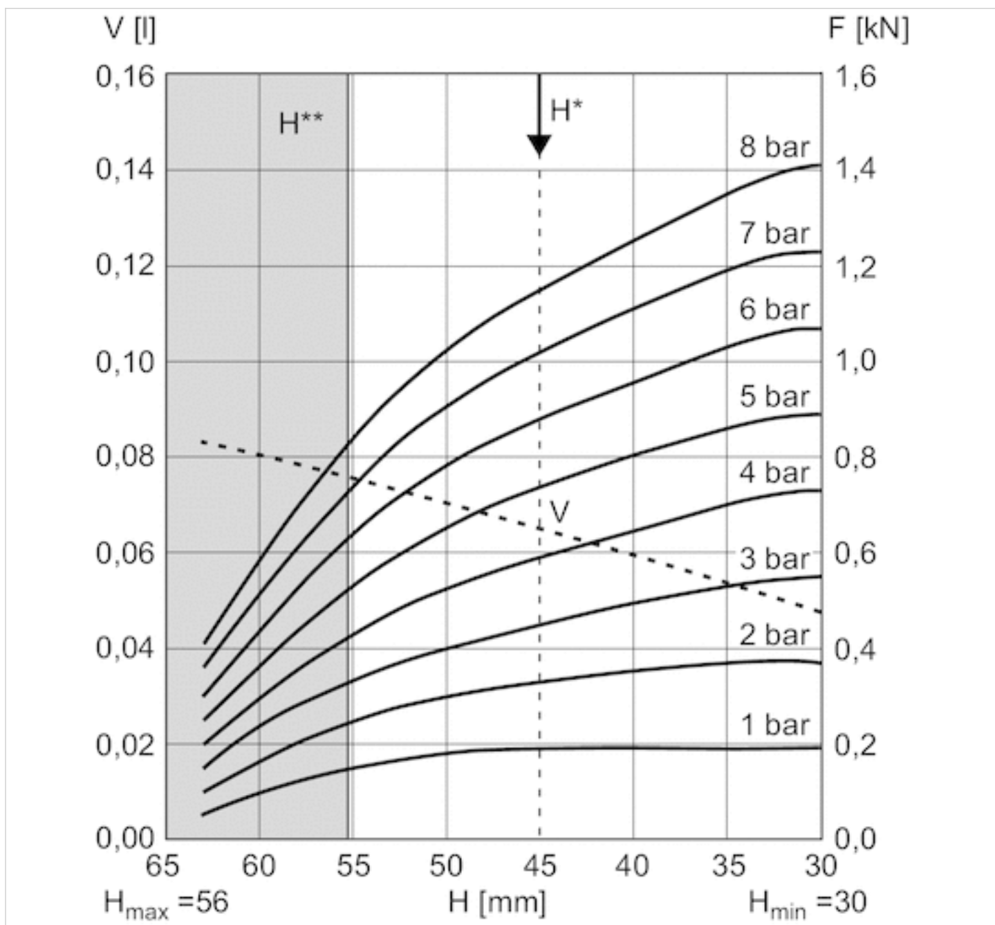
Force-displacement diagram, 2719060300
